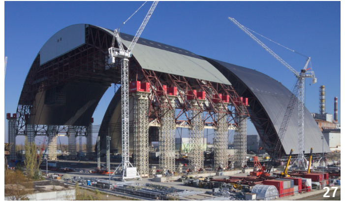
October 2014: Third and final lifting operation for the second half of the arch.
